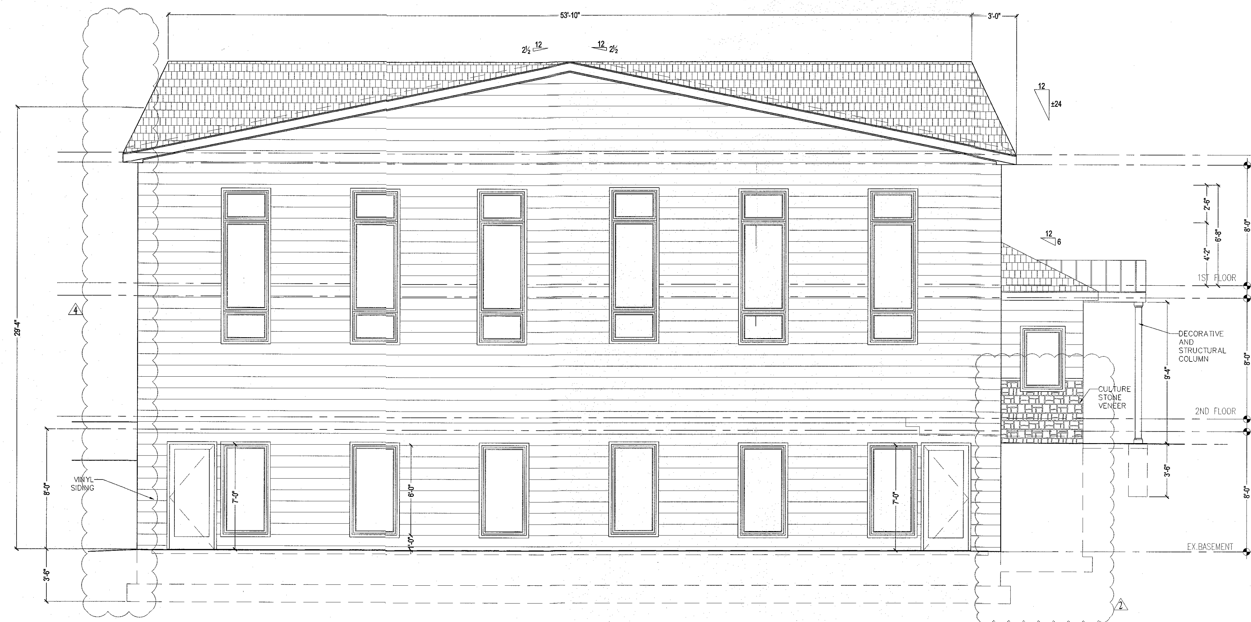
WEST ELEVATION - REAR SCALE: 1/4"=1'-0"
