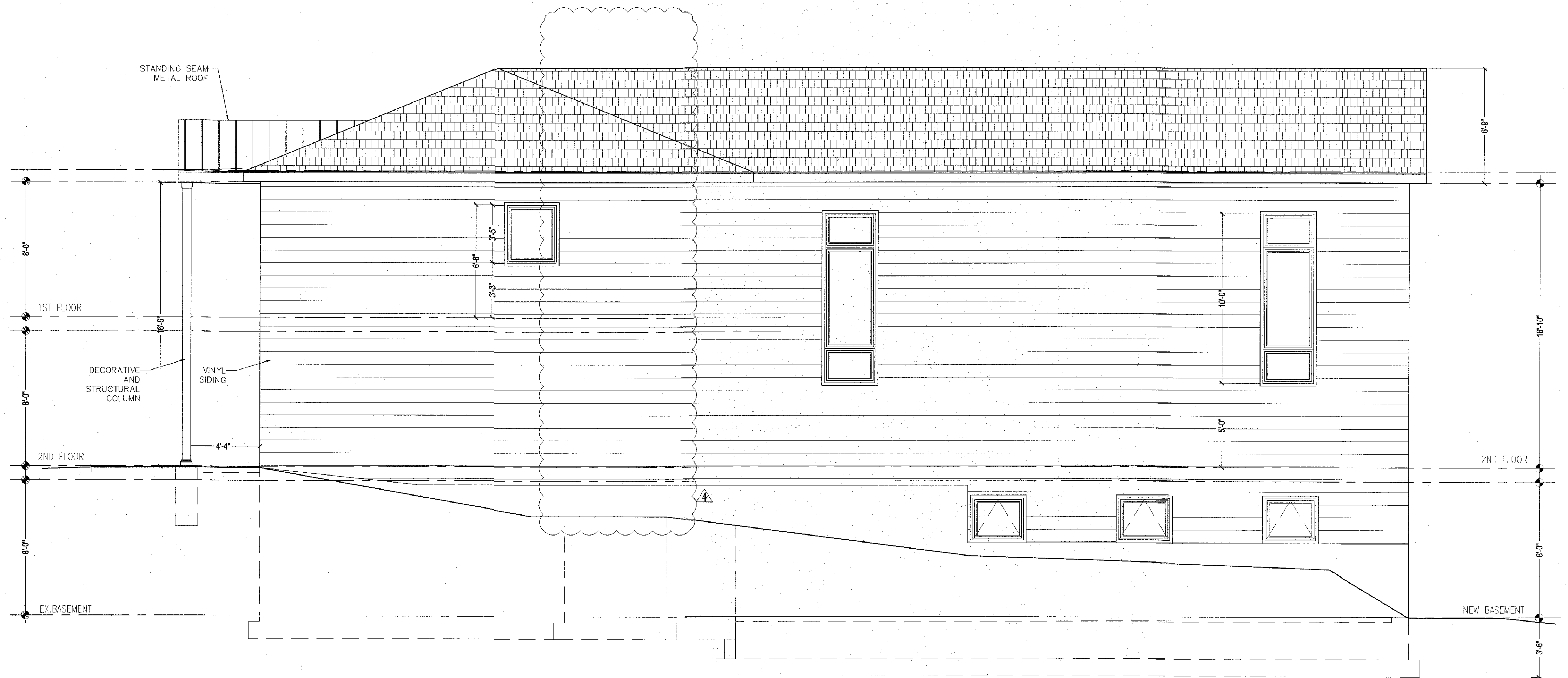
NORTH ELEVATION - RIGHT
